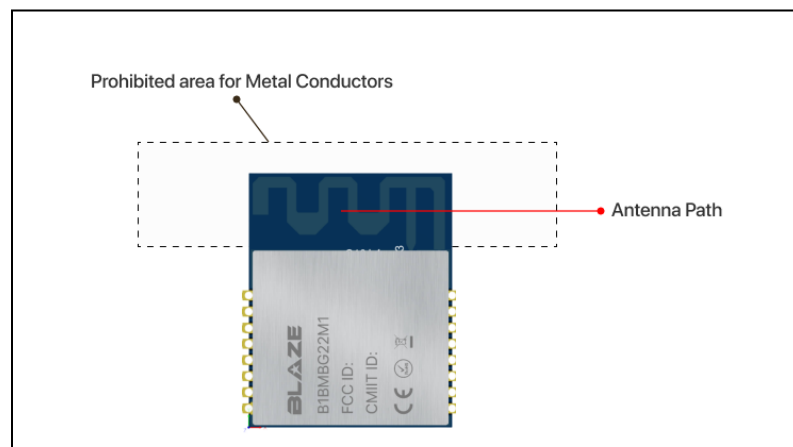
Figure 10.4. Antenna portion away from metal
