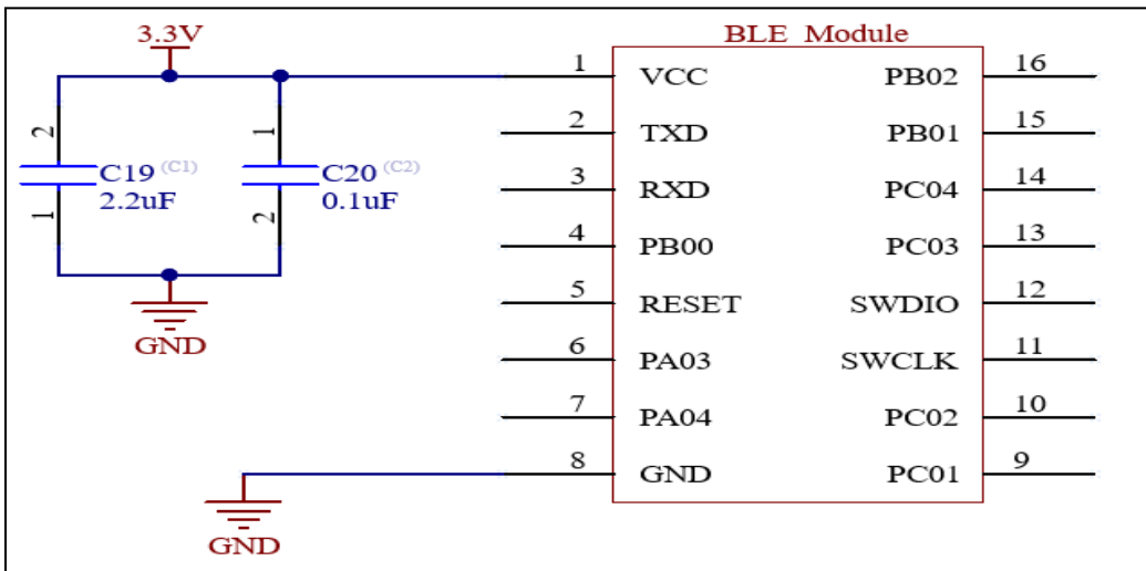
Figure 6.1. Reference Design of BLE module B1BMBG22M1
