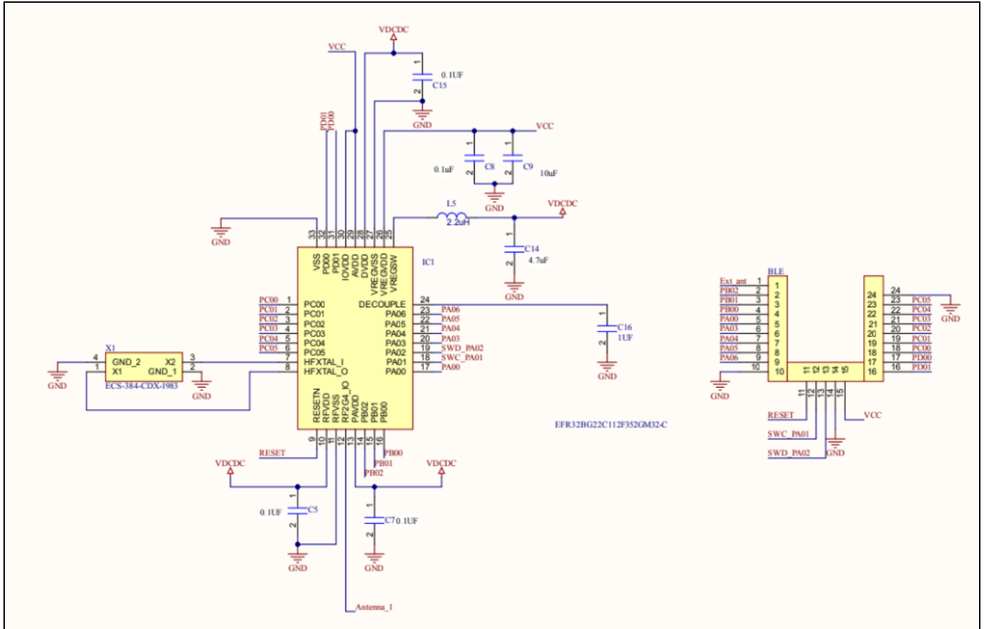
Figure 9.2. Schematic Diagram of BLE Module
