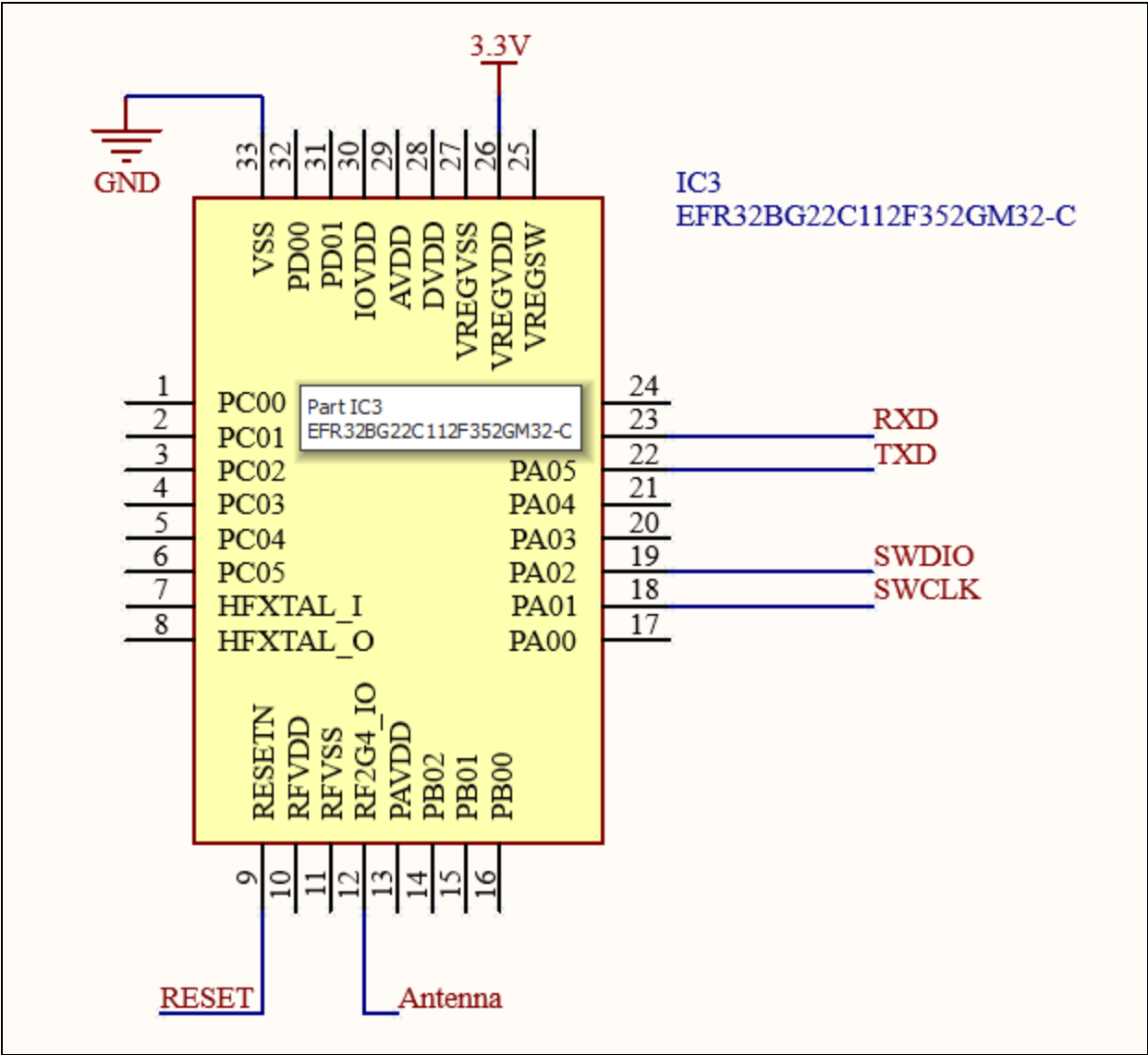
Figure 7.1. Stand-alone SoC configuration for SoC EFR32BG22C112F352GM32-C
