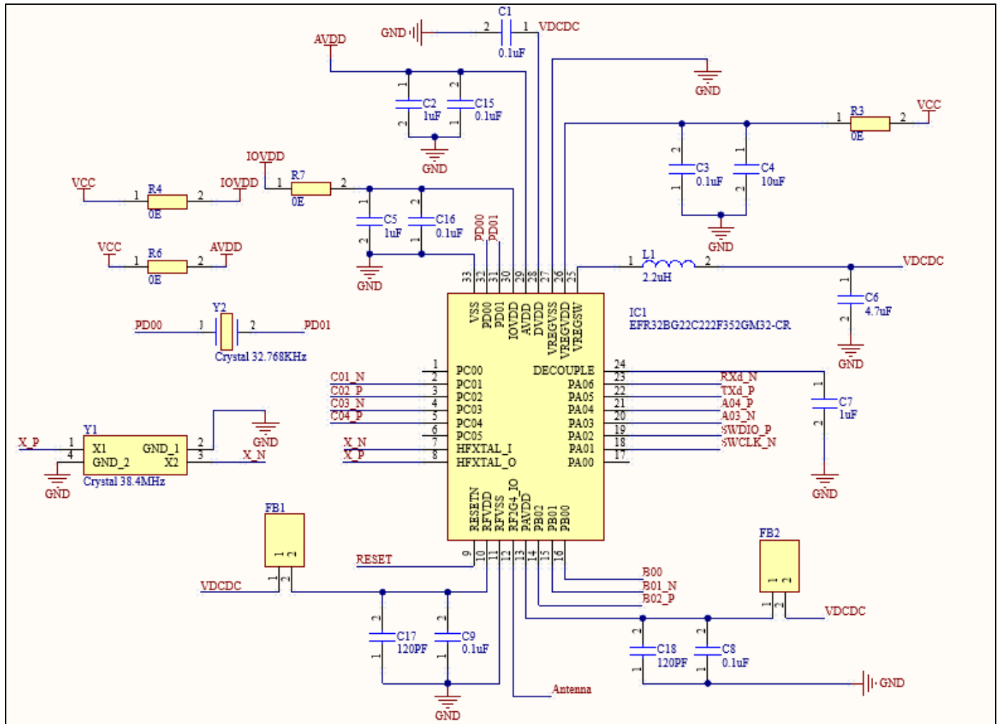
Figure 9.1. Schematic Diagram of BLE Module B1BMBG22M1
