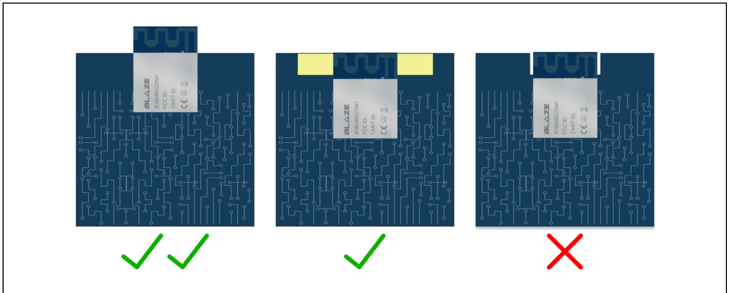
Figure 10.5 Module Placement for module B1BMBG22M1
