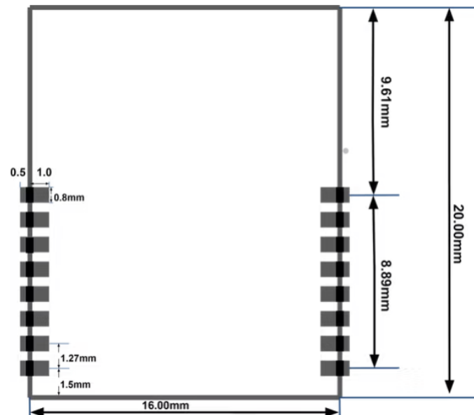
Figure 11.1. Dimensions of PCB
