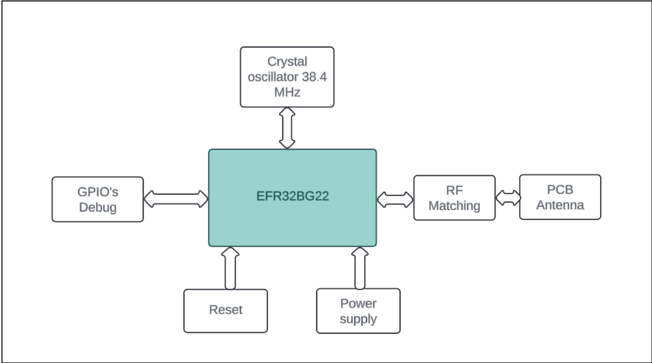
Figure 3.1. Block Diagram of BLE Module B1BMBG22M1
