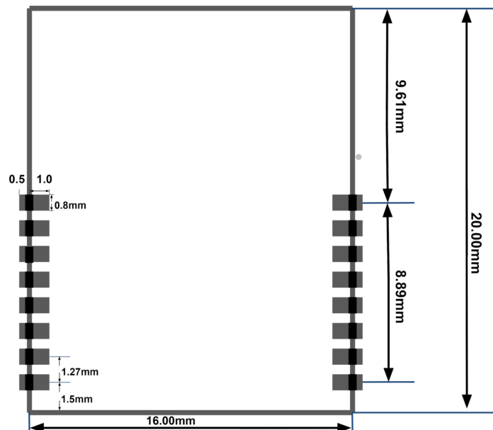
Figure 11.2. Recommended PCB Footprint of BLE Module B1BMBG22M1
