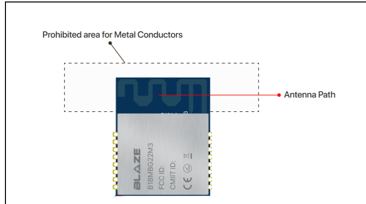
Figure 10.4. Antenna portion away from metal
