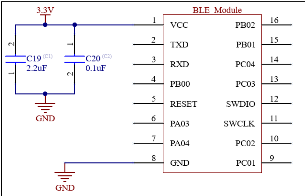
Figure 6.1. Reference Design of BLE module B1BMBG22M3
