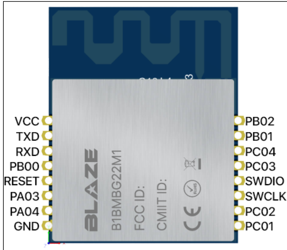
Figure 5.1. PIN Diagram of BLE Module B1BMBG22M3
