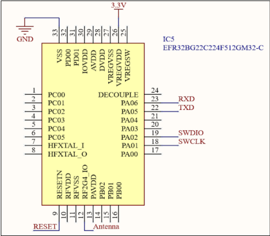
Figure 7.1. Stand- alone SoC configuration for SoC EFR32BG22C224F512GM32-C
