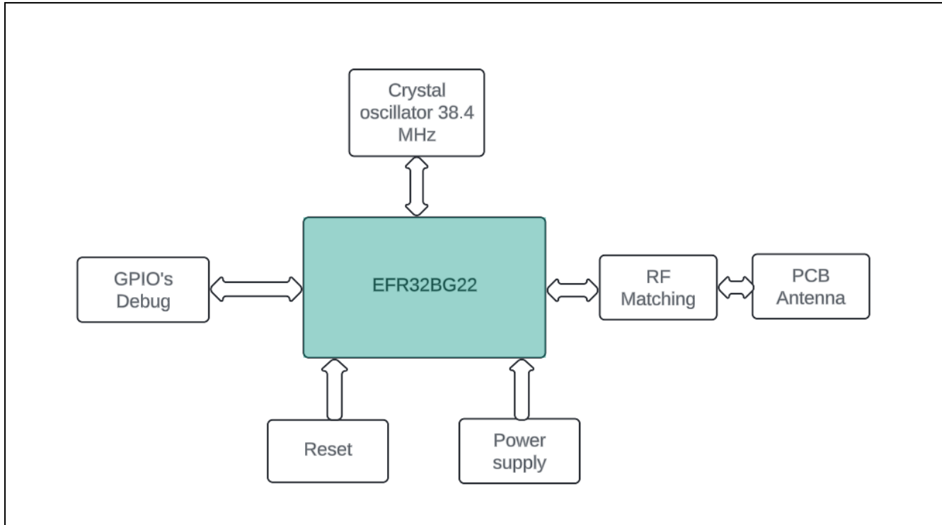
Figure 3.1. Block Diagram of BLE Module B1BMBG22M3
