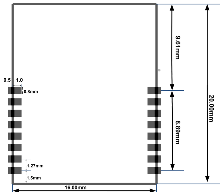
Figure 11.2. Recommended PCB Footprint of BLE Module B1BMBG22M3
