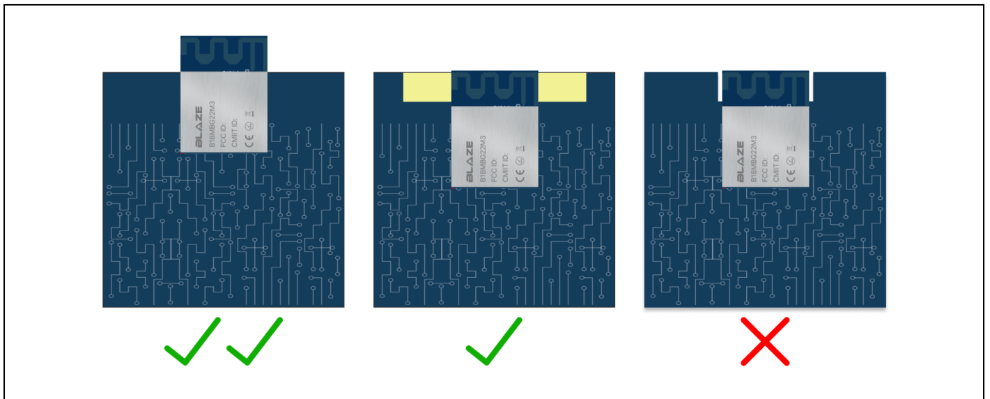
Figure 10.5 Module Placement for module B1BMBG22M3
