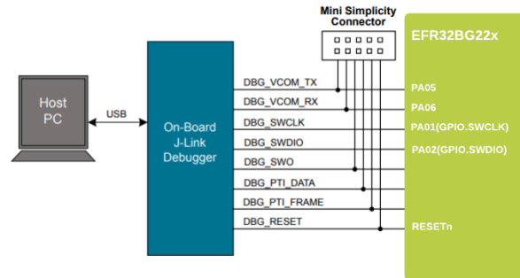
Figure 2.4 Onboard debugging connections
