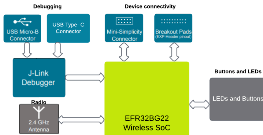
Figure 2.1 Kit Block diagram
