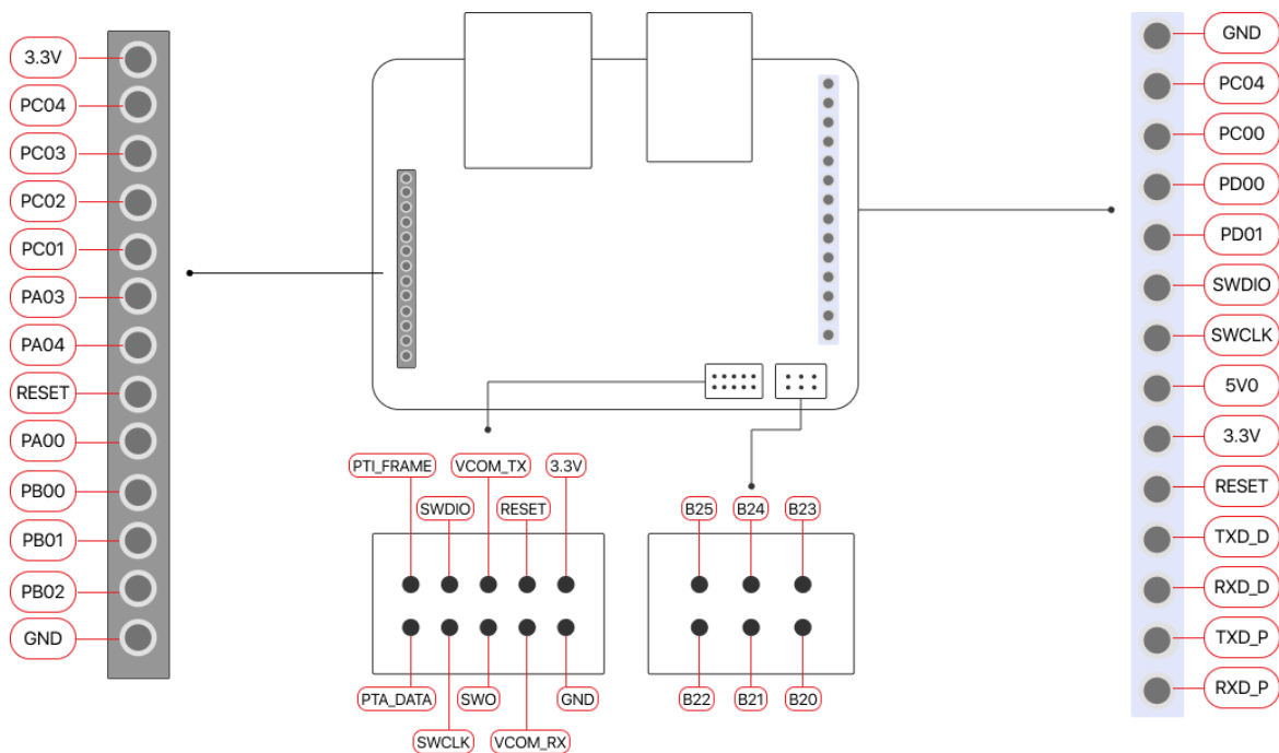
Figure 2.5 BLE Dev Kit Connectors
