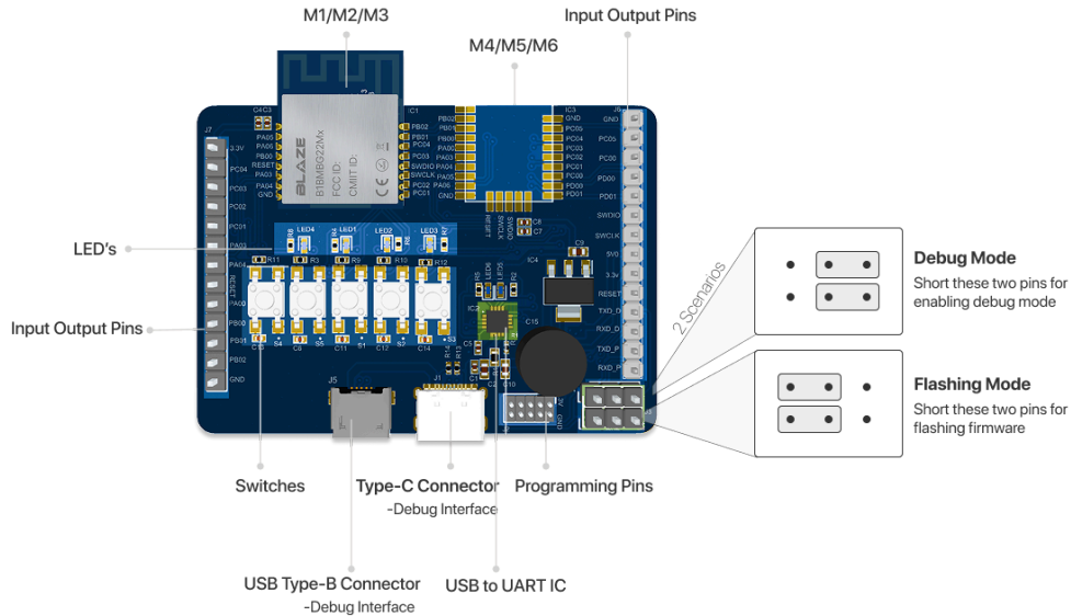
Figure 1.1 BLE Dev kit hardware layout
