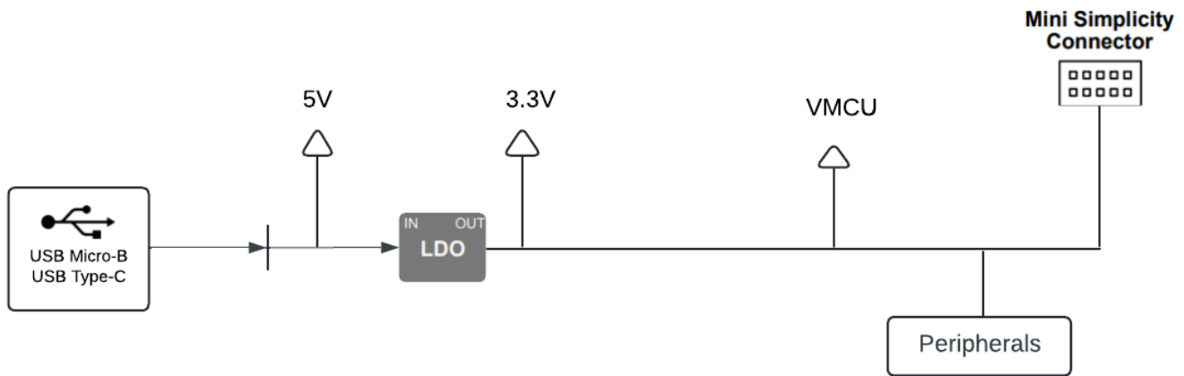
Figure 2.2 BLE Dev Kit power architecture
