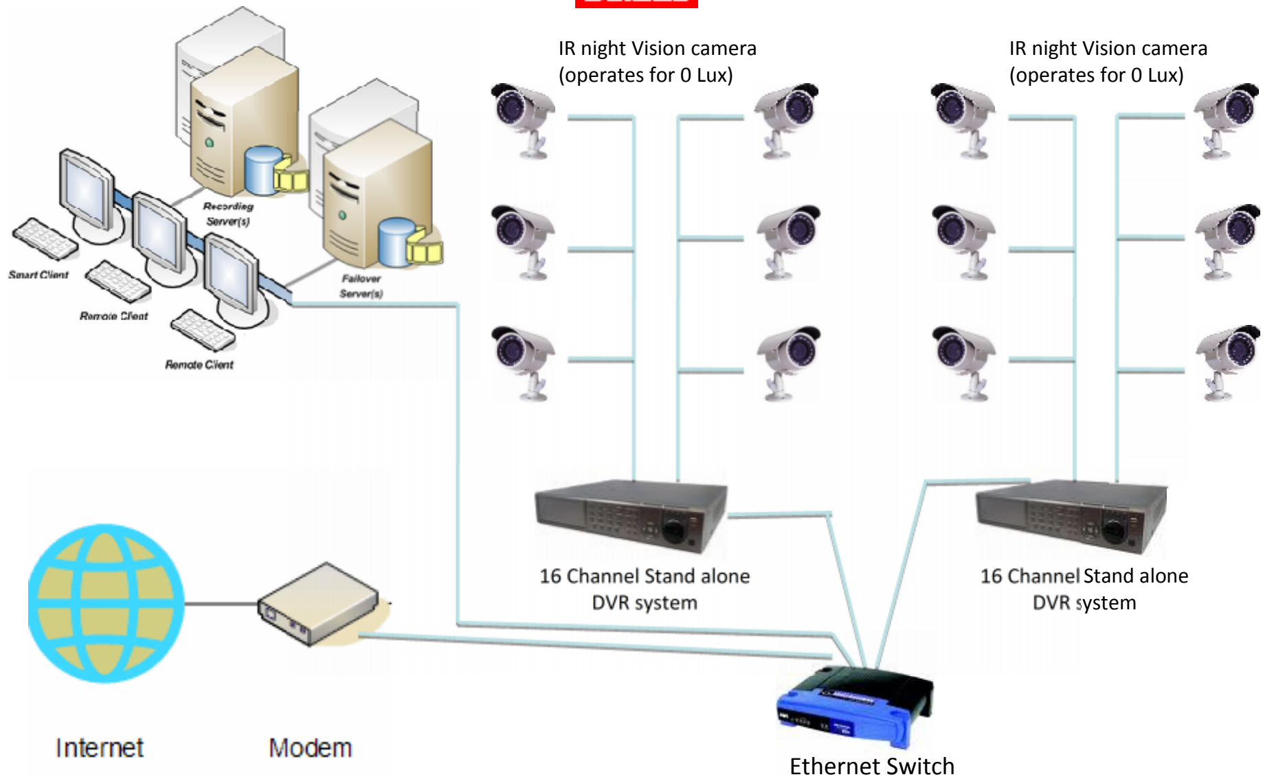
Typical Architecture of CCTV camera based Surveillance system
